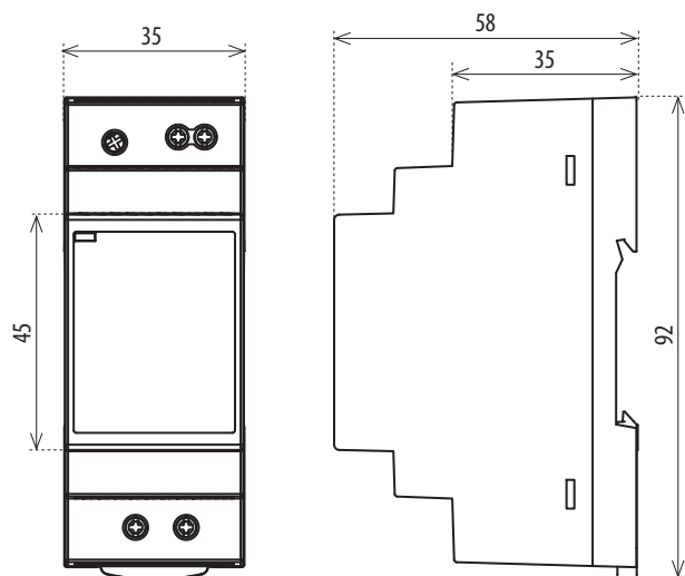
PS2M-24/12V PS2M-30/24V
